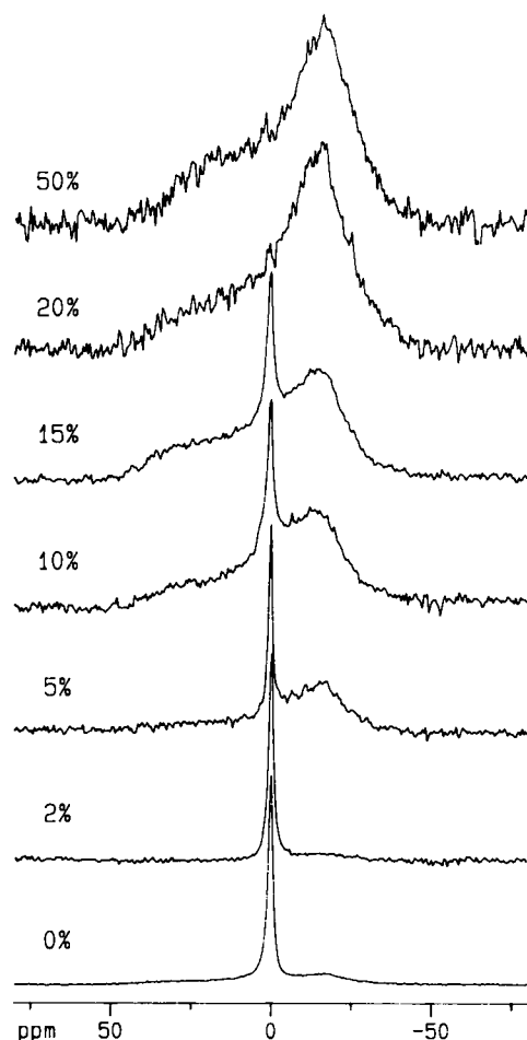
FIGURE 1 ^{31}\text{P} -NMR spectra of DPPG/DPPC mixtures in the presence of melittin at R_i = 40 , pH = 7.5, at 26°C. DPPG molar concentration is indicated for each spectrum.
