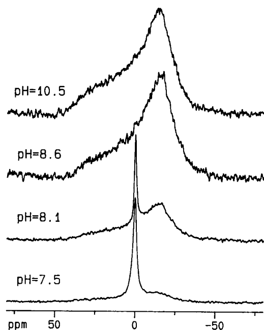
FIGURE 3 ^{31}P -NMR spectra of a DPPC sample containing 10 mol % palmitic acid in the presence of melittin at R_i = 60 at 26^\circ C as a function of the pH .
