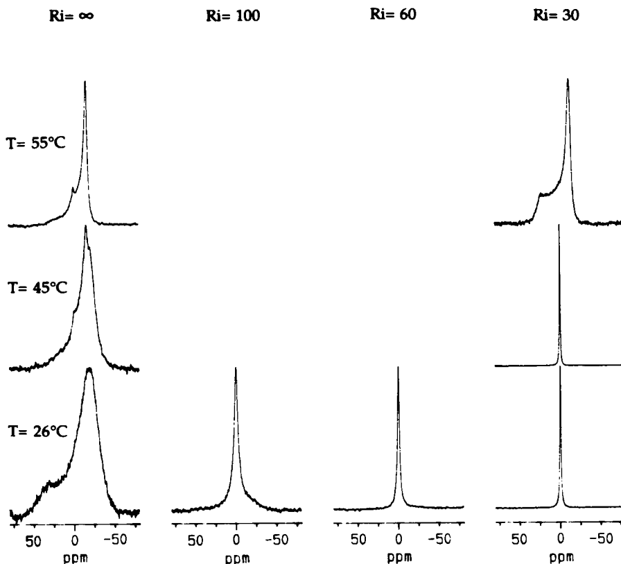
FIGURE 5 ^{31}\text{P} -NMR spectra of a DPPC/10 mol % DPTAP mixture at various temperatures (26, 45, and 55°C) and various lipid/melittin R_i 's at pH = 7.5.
