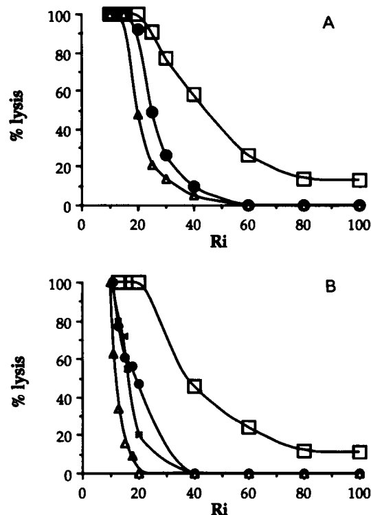
FIGURE 2 Relative amount of lysis with respect to the lipid/peptide R_i at 26°C for 10 mol % DPPG ( \blacktriangle ) or DMPS ( \bullet ) in DPPC and pure DPPC ( \square ) at pH = 7.5 (A), and for 10 mol % palmitic acid ( \blacktriangle ), oleic acid ( * ), or linoleic acid ( \bullet ) in DPPC and pure DPPC ( \square ) at pH = 9.5 (B).
